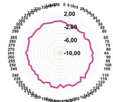
Freq. 1800 MHz H-plane (dBi) V-pol
