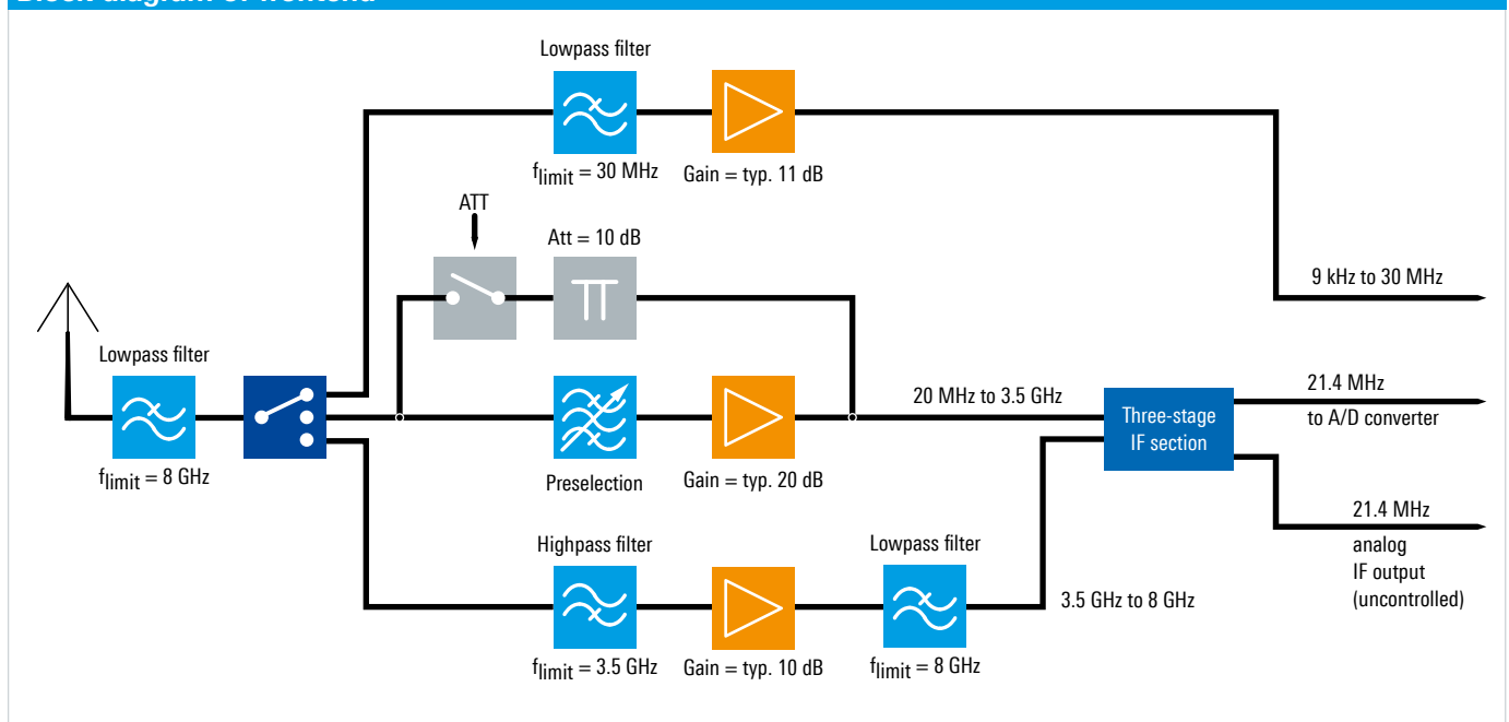
Block diagram of frontend
